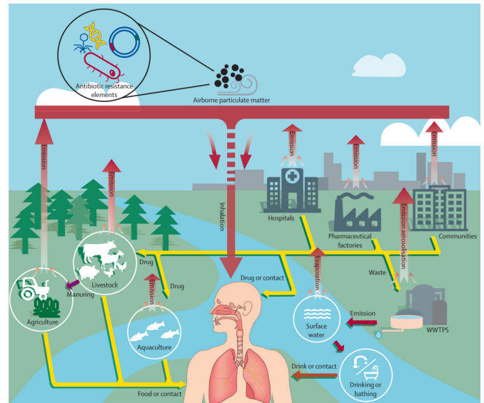
Figura 2. Pathways of antibiotic-resistance dissemination WWTPs=waste water treatment plants. (Fonte: 13)
